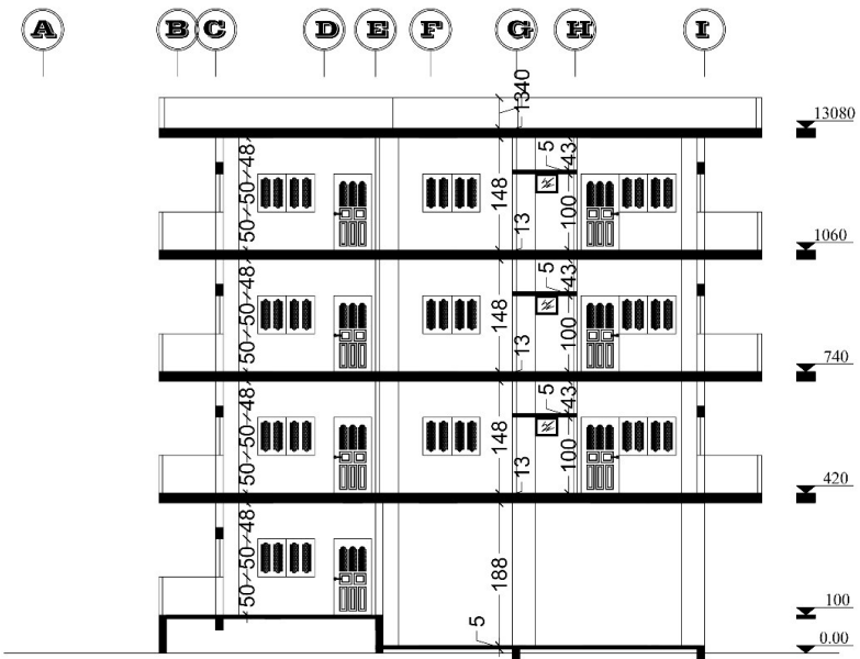
BB' section
