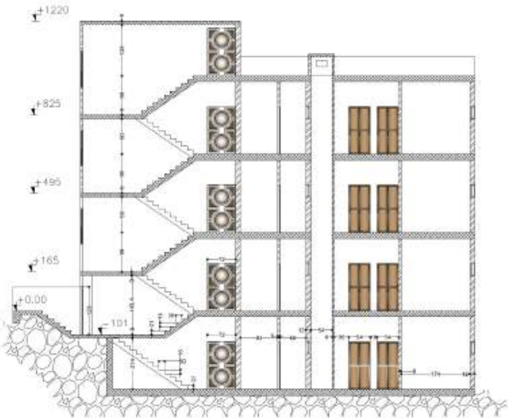
BB' section
