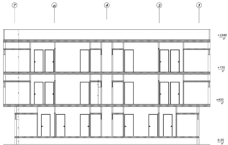
BB' section
