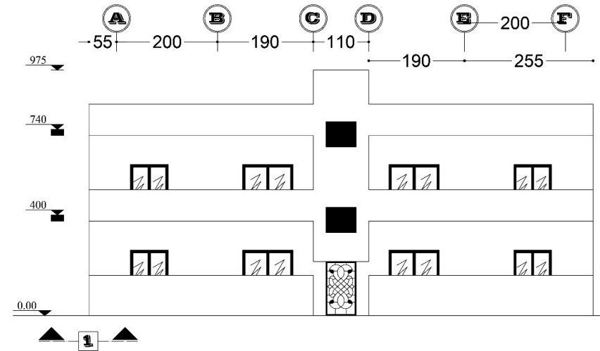
Southern Elev.
