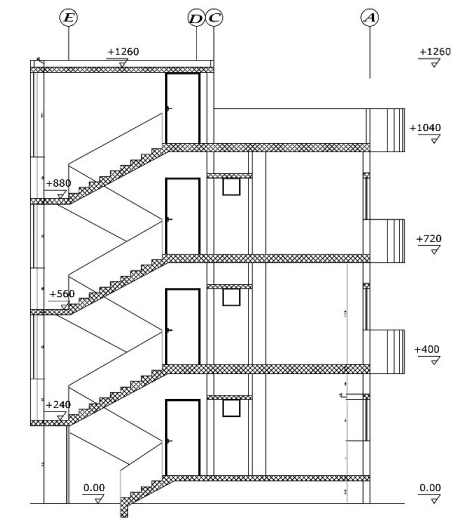
AA' section
