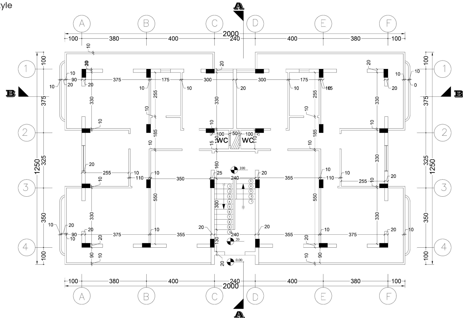
Ground floor
