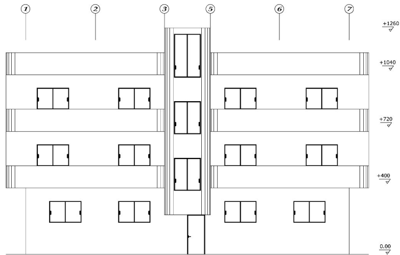
Southern Elev.
