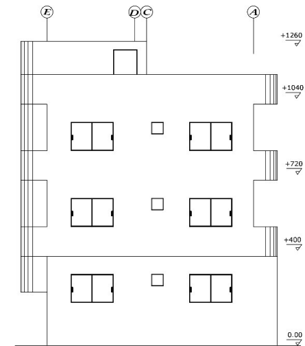
Western Elev.
