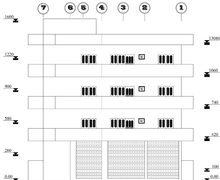
Eastern Elev.
