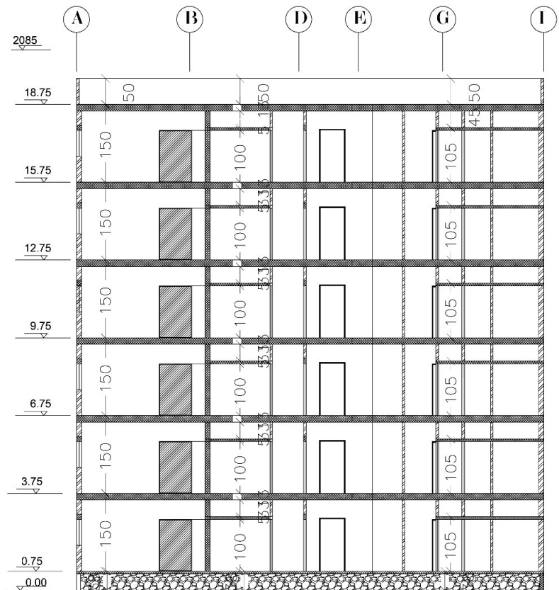
BB' Section
