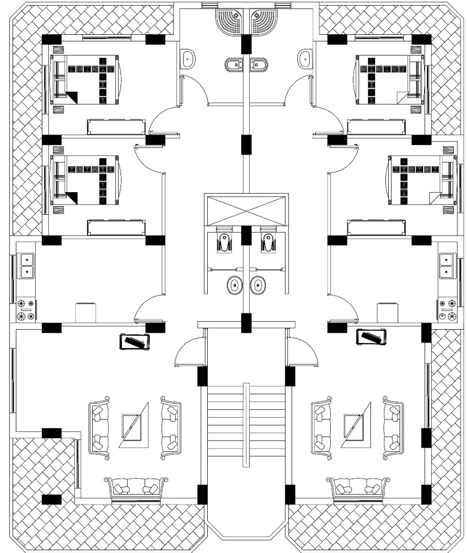
2 nd floor
