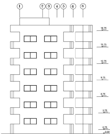
Southern Elv.
