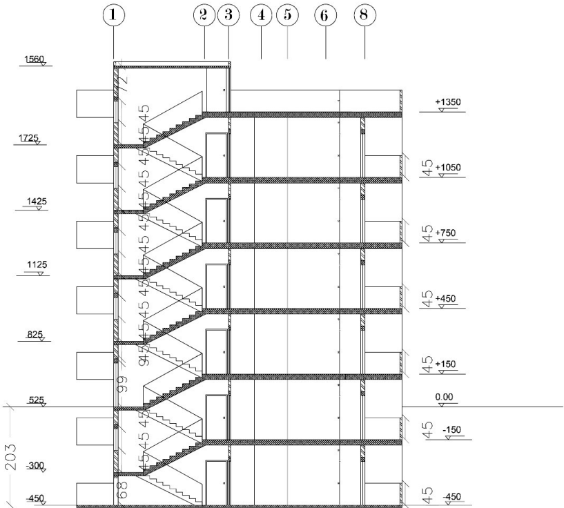
BB' section
