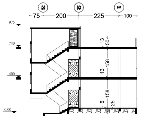
BB' section
