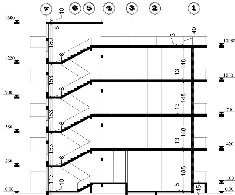
AA' section
