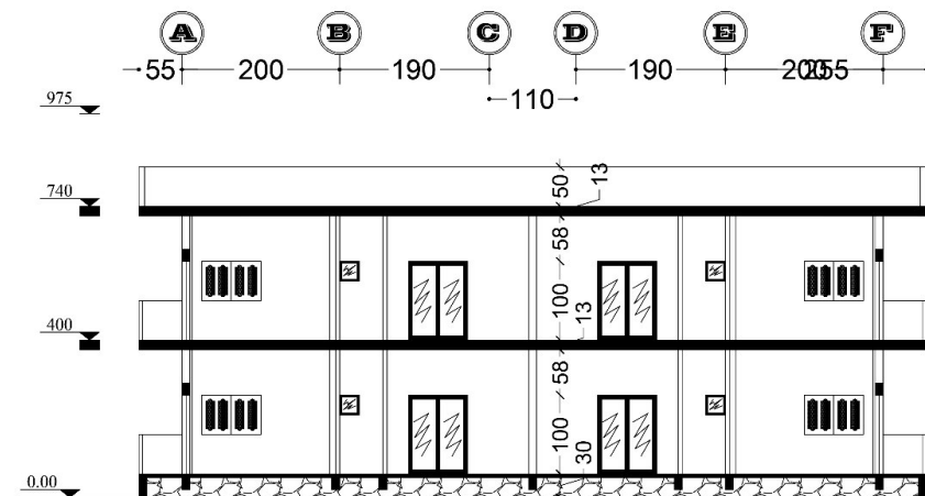
AA' section
