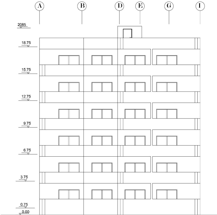
Weastern Elv.
